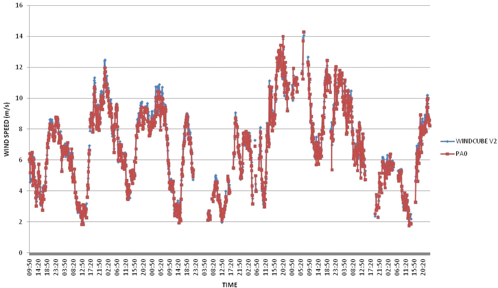
PA 0 / WindCube V2 (1032 ten minutes time steps ~ 9 days) WIND SPEED TIME SERIES 130 m 28 OCT - 05 NOV 2015 AT BOURGES PROVING GROUND
